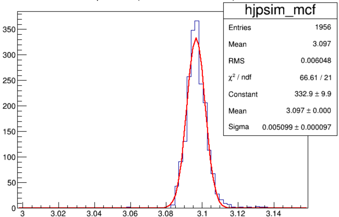
J/ψ mass (mass constraint fit)
