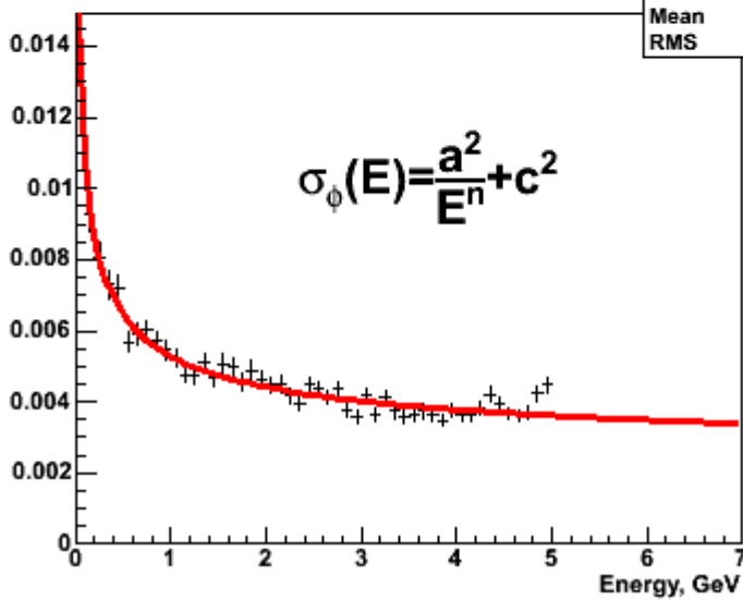
Phi difference (barrel)
