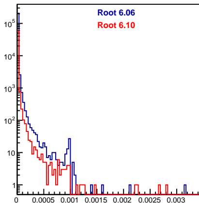
MdtPoint.fELoss {MdtPoint.fZ&lt;400}
