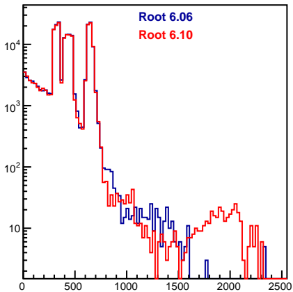
FTSPoint.fLength
