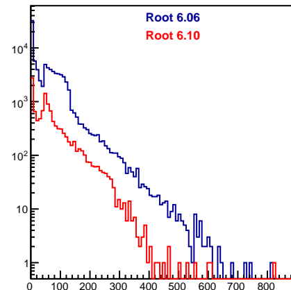
DrcBarPoint.fLength
