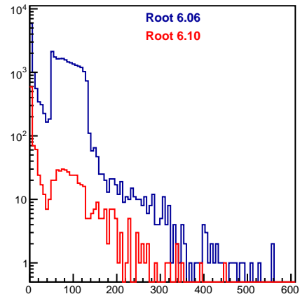
SciTPoint.fLength
