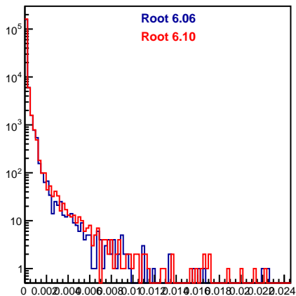
MVDPoint.fELoss
