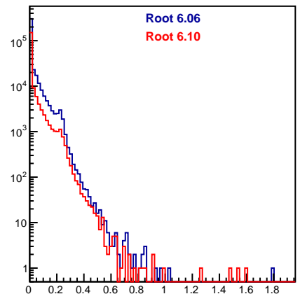
EmcHit.fEnergy
