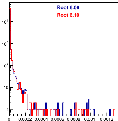
MdtPoint.fELoss {MdtPoint.fZ&gt;800}
