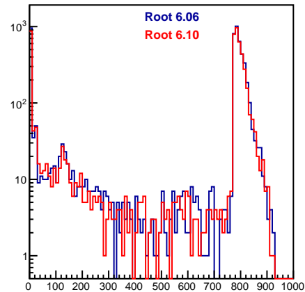
FtofPoint.fLength
