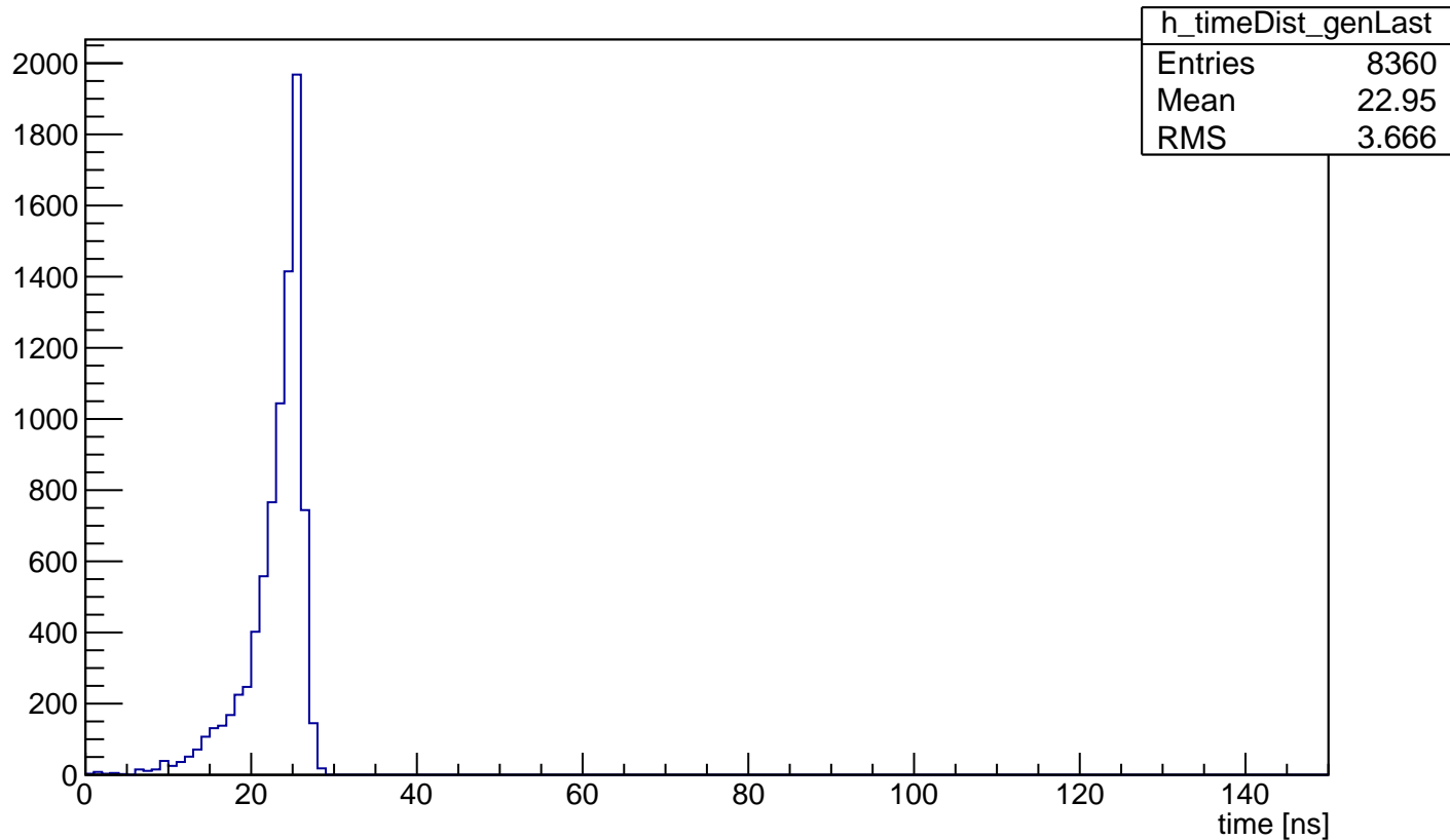
time stamp distribution of generator last particles in Ftof
