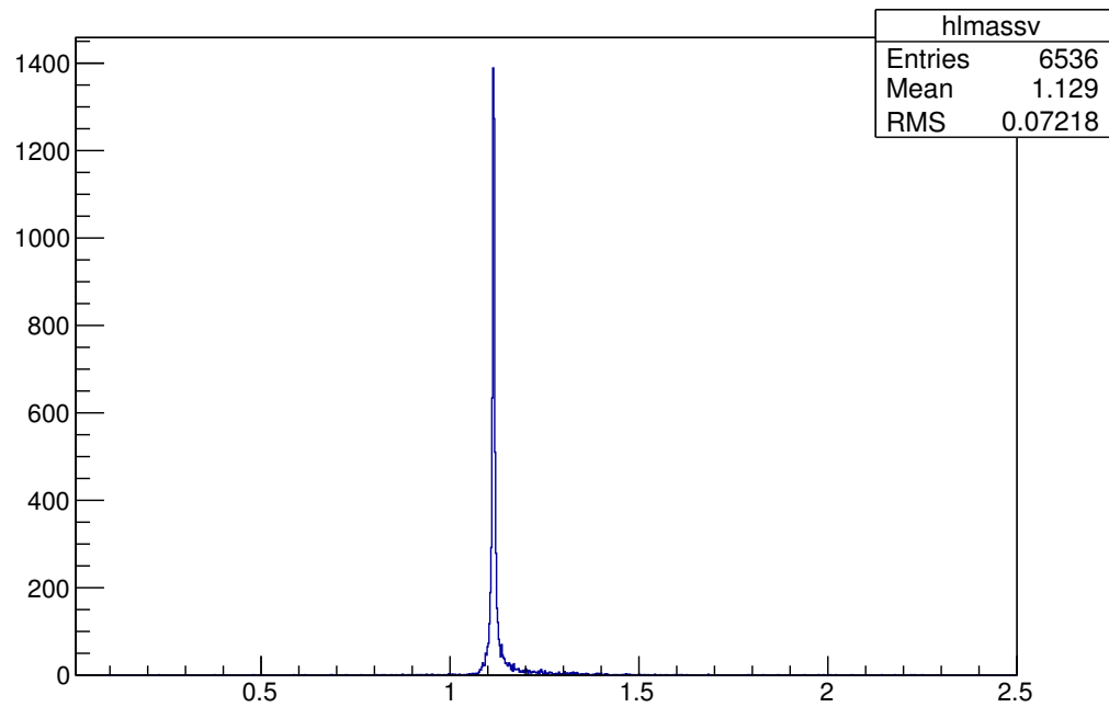
lambda cand vertex fit
