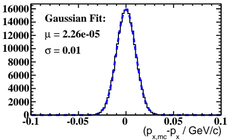
Momentum Smearing
