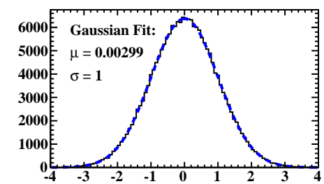
PRG Pull Distribution (2)
