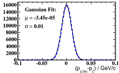
Momentum Smearing
