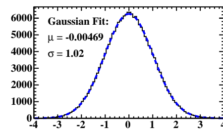
PRG Pull Distribution (1)
