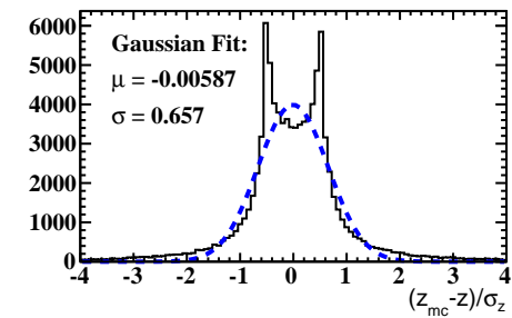
Vertex pull distribution POCA
