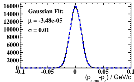
Momentum full kin
