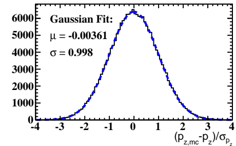
Momentum pull distribution reco
