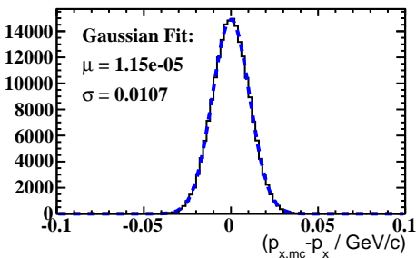
Momentum full fit
