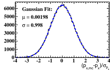
Momentum pull distribution reco
