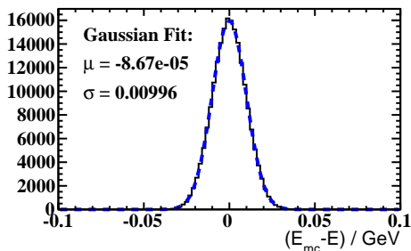
Energy reco
