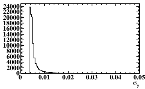
Vertex error distribution fast
