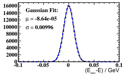
Energy full kin
