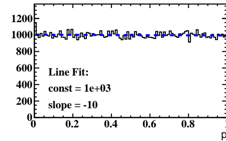
P(\chi^2) Fit
