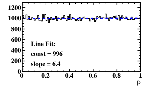
P(\chi^2) Kin
