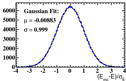
Energy pull distribution full fit
