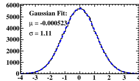
PRG Pull Distribution (0)
