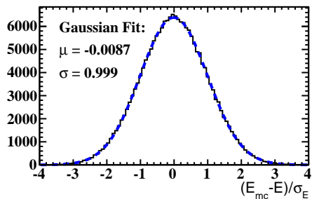
Energy pull distribution reco
