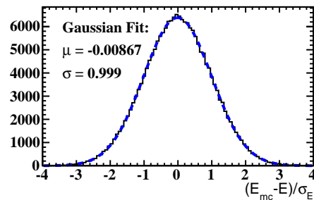
Energy pull distribution full kin
