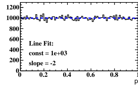
P(\chi^2) Fast
