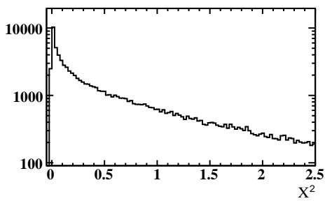
Vertex Fast \chi^2
