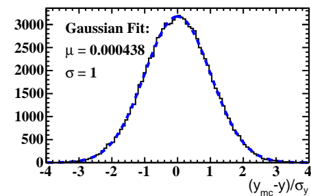
Vertex pull distribution fast
