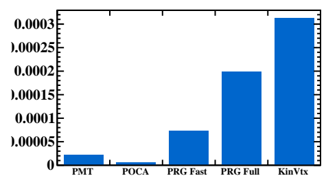
CPU loads
