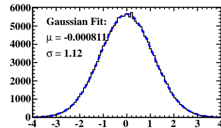
PRG Pull Distribution (3)
