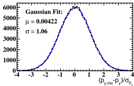
Momentum full kin
