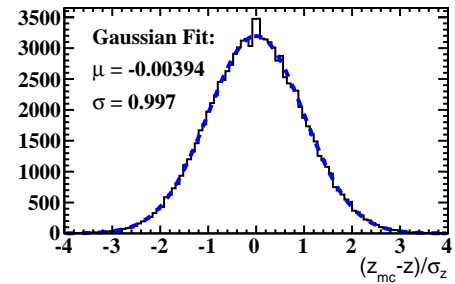
Vertex pull distribution full kin
