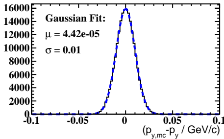
Momentum Smearing
