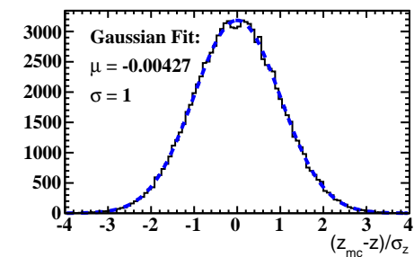
Vertex pull distribution fast
