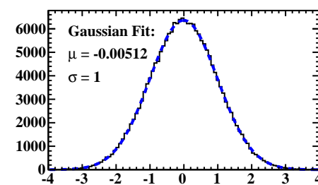
PRG Pull Distribution (4)
