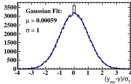
Vertex pull distribution full kin
