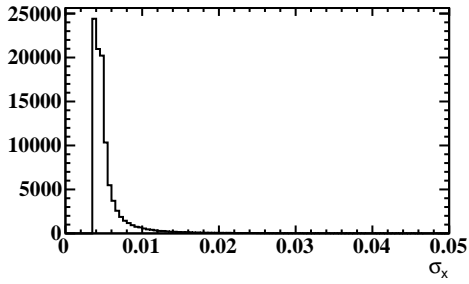
Vertex error distribution full fit
