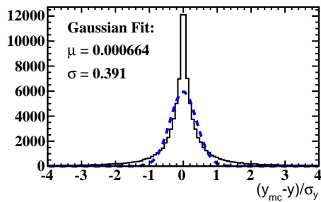
Vertex pull distribution POCA
