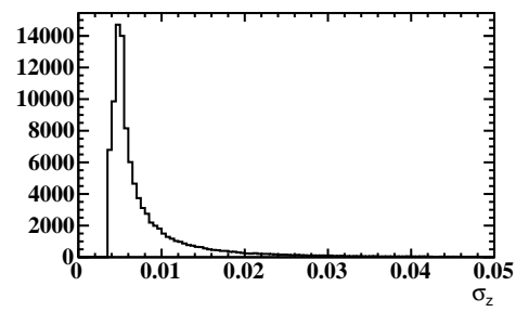
Vertex error distribution fast
