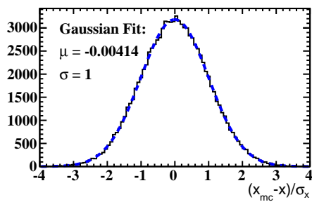
Vertex pull distribution full fit
