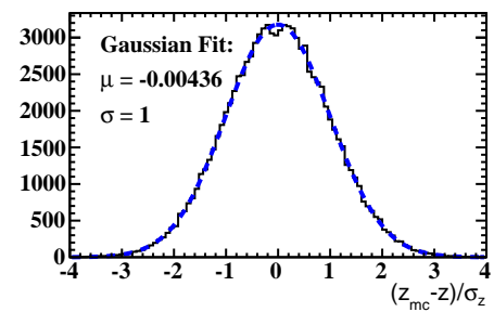
Vertex pull distribution full fit
