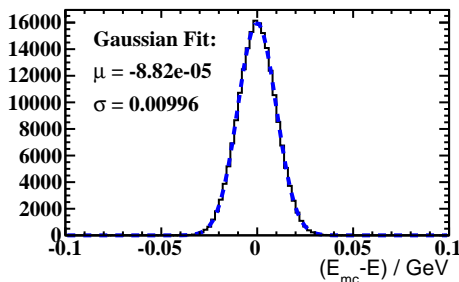
Energy full fit
