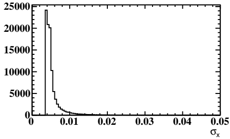
Vertex error distribution full kin
