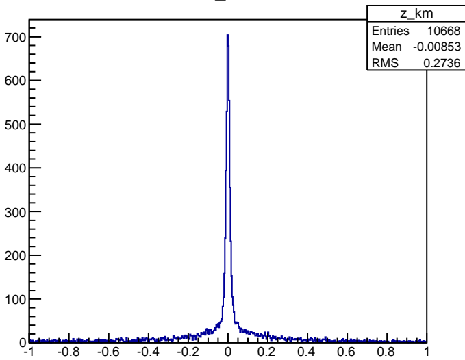
z_km
