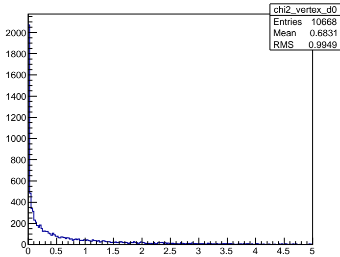
chi vertex
