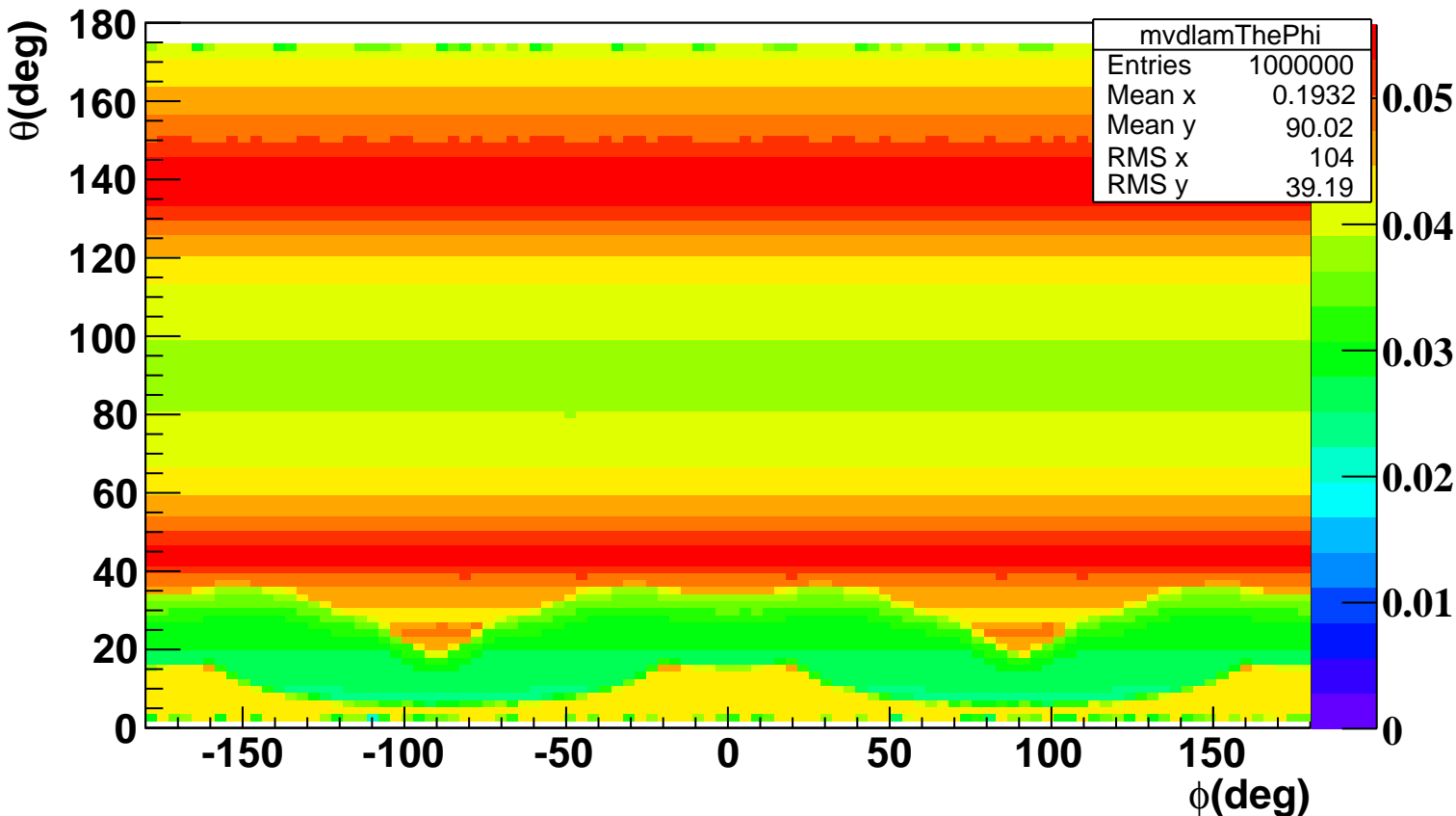
Radiation length map [x/x0] \theta & \phi
