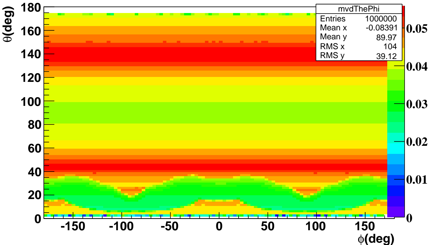
Radiation length map [x/x0] \theta & \phi
