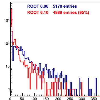
FtofPoint.fTrackID
