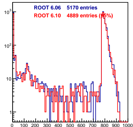
FtofPoint.fLength
