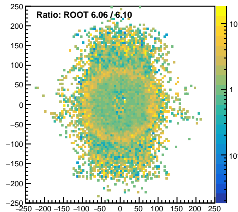
MCTrack.fStartX:MCTrack.fStartY (fStartZ&gt;200)
