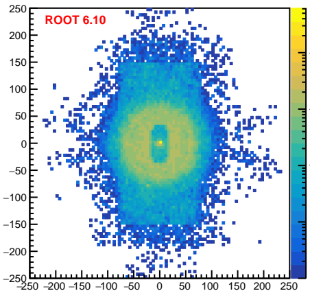
MCTrack.fStartX:MCTrack.fStartY
