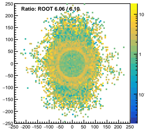
MCTrack.fStartX:MCTrack.fStartY
