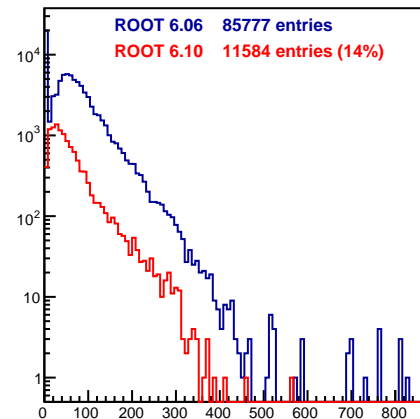
DrcBarPoint.fTrackID
