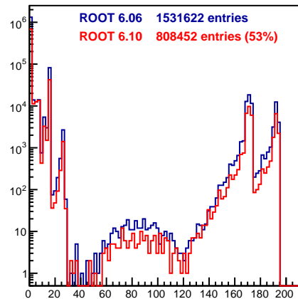
MCTrack.fE
