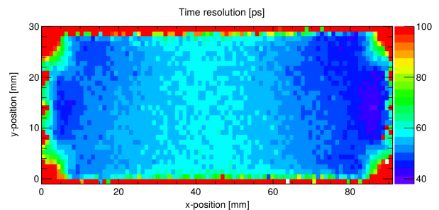
Figure 6: Time resolution distribution along the surface of a 90 \times 30 \times 5 \text{ mm}^3 EJ-232 scintillator. The average was \sim 54 ps.
