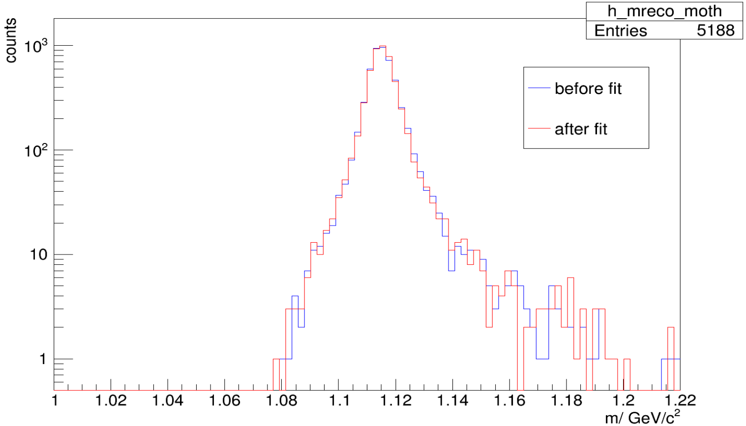
Mass of Lambda0 before Fit
