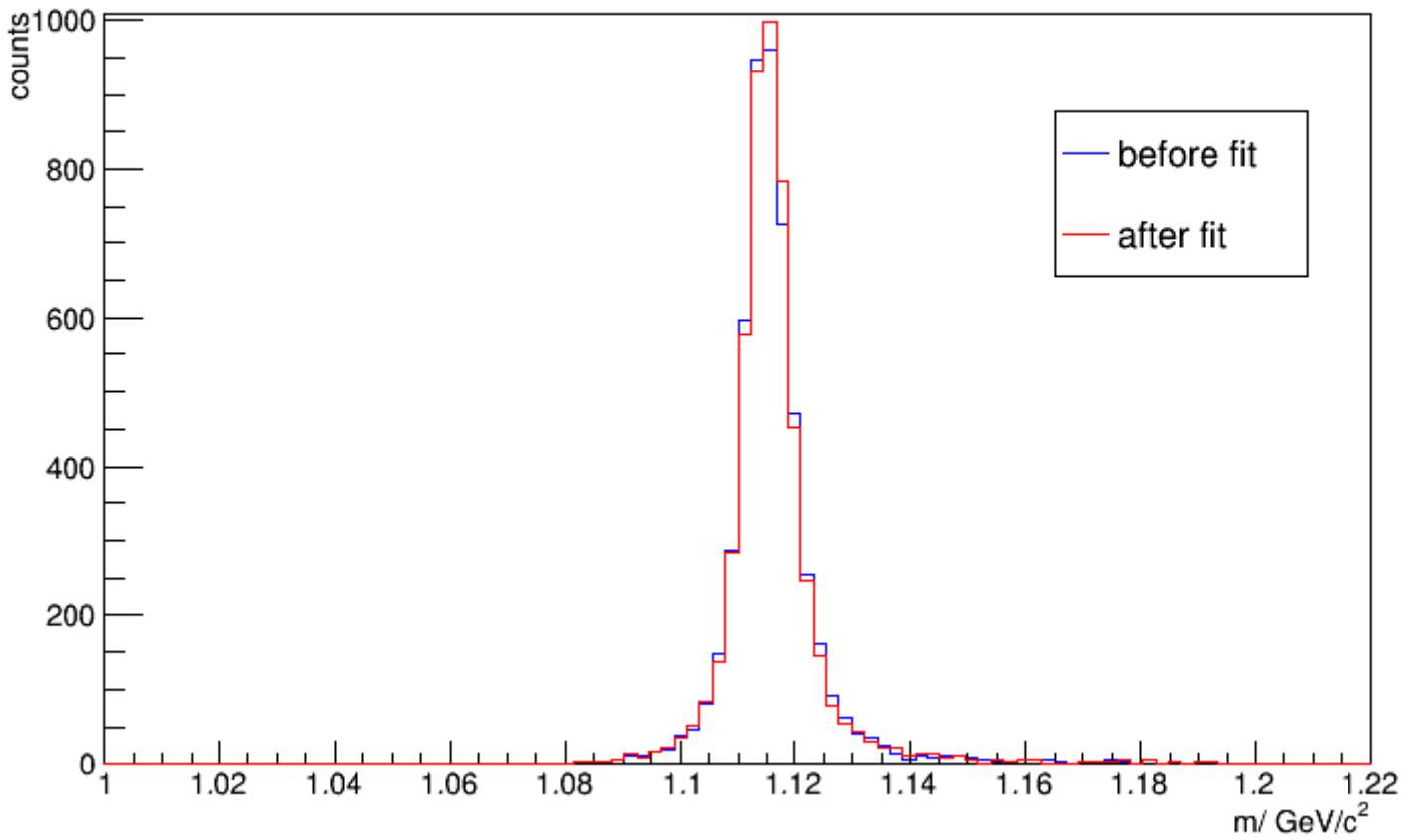
Mass of Lambda0 before Fit
