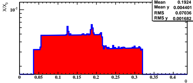
Effective radiation length ( X/X_0 ) vs \theta
