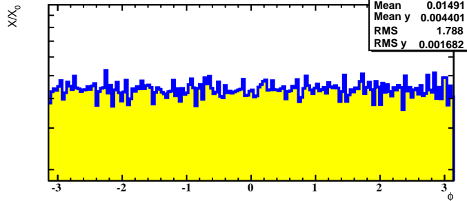
Effective radiation length ( X/X_0 ) vs \phi
