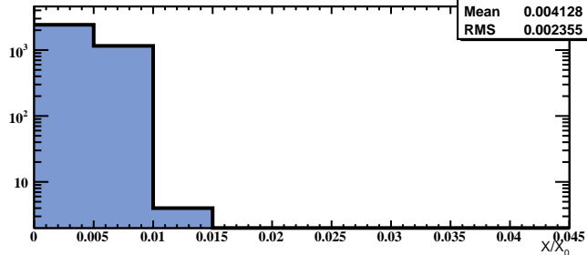
Effective radiation length ( X/X_0 )
