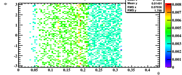
Effective radiation length ( X/X_0 ) vs \theta & \phi
