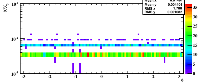
Effective radiation length ( X/X_0 ) vs \phi
