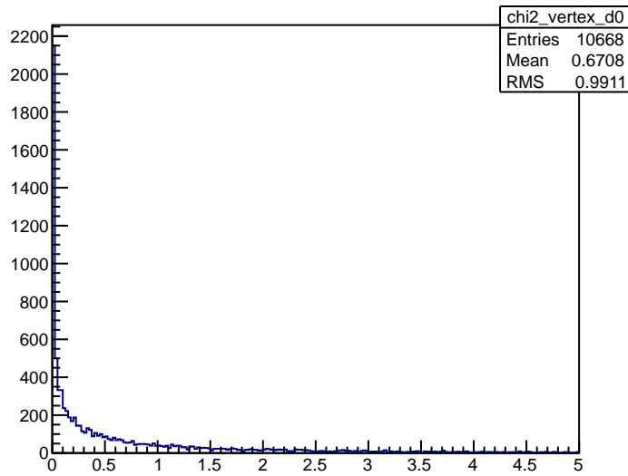
chi vertex
