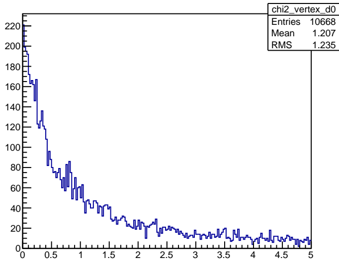
chi vertex
