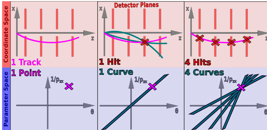
Figure 2: Illustration of the basic principle for a Hough transform using a parabola track model for a toy detector.
