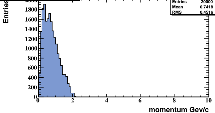
momentum of Pions from MC
