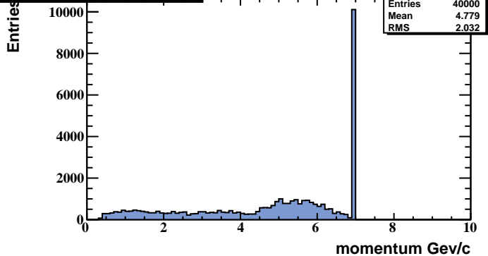
momentum of Electrons from MC
