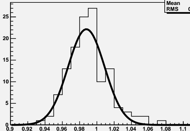
Kalman total momentum for \mu^+
