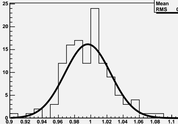
Total momentum for \mu^+
